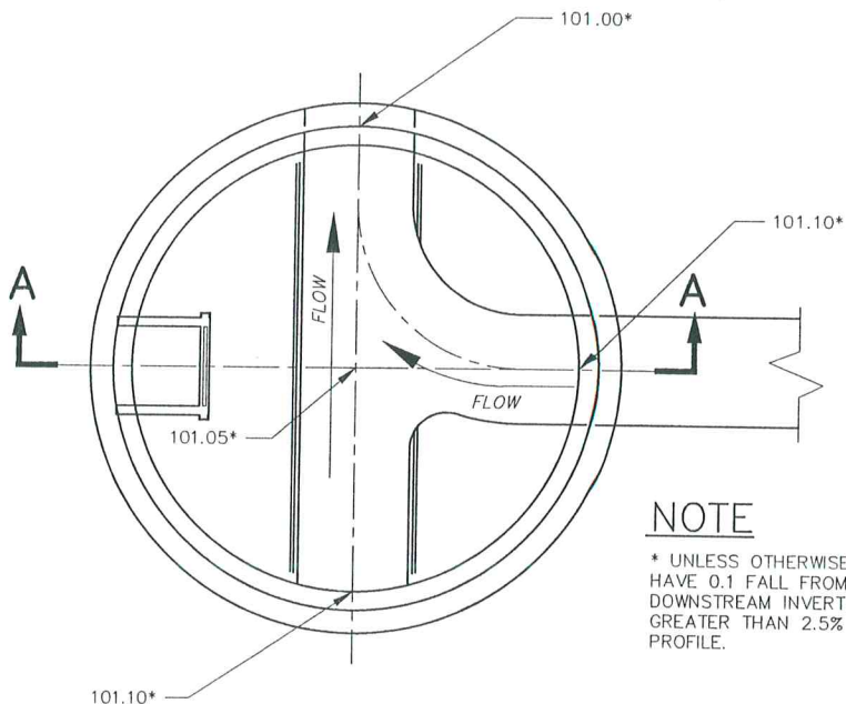
PLAN VIEW 48" ID CHANNELLED BASE N.T.S.
