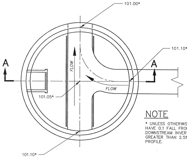
PLAN VIEW 48" ID CHANNELED BASE N.T.S.
